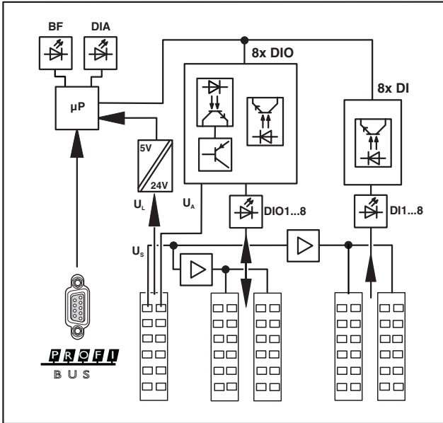
Figure 2 Internal wiring of the terminal points
