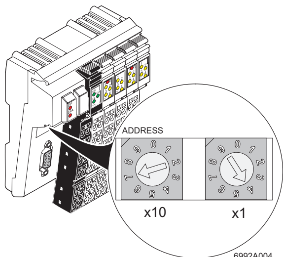
Figure 4 PROFIBUS rotary encoding switches
