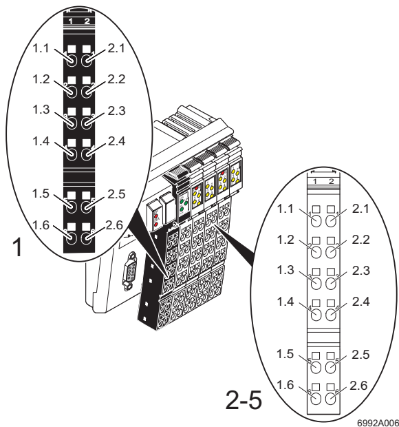
Figure 6 Terminal point assignment of Inline connectors (module version ILB PB 24 DI8 DIO8 as an example)
