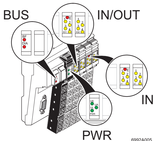
Figure 3 Diagnostic and status indicators of the ILB PB 24 DI8 DIO8 (/CN) module
