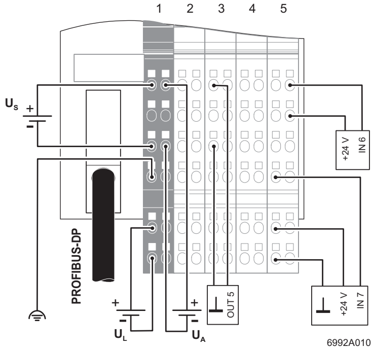
Figure 7 Connection example
