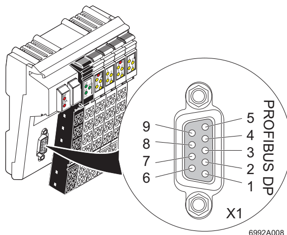
Figure 5 Pin assignment of the 9-pos. D-SUB female connector
