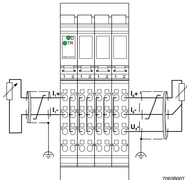
Figure 5 Connection of sensors in 2 and 3-wire technology with shield connection
