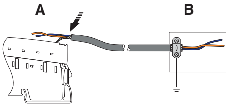
Figure 4 Connection of analog sensors using a multi-wire bus cable
