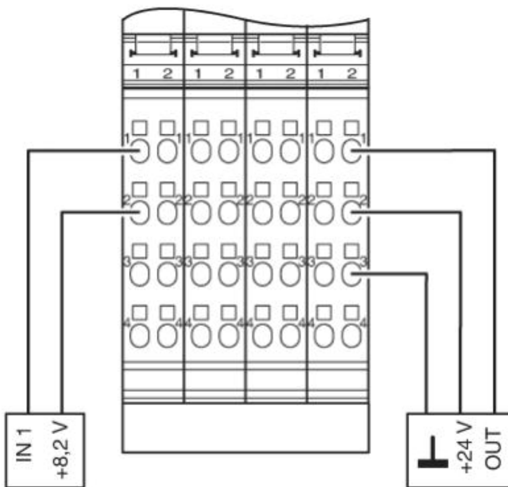
Connection diagram
