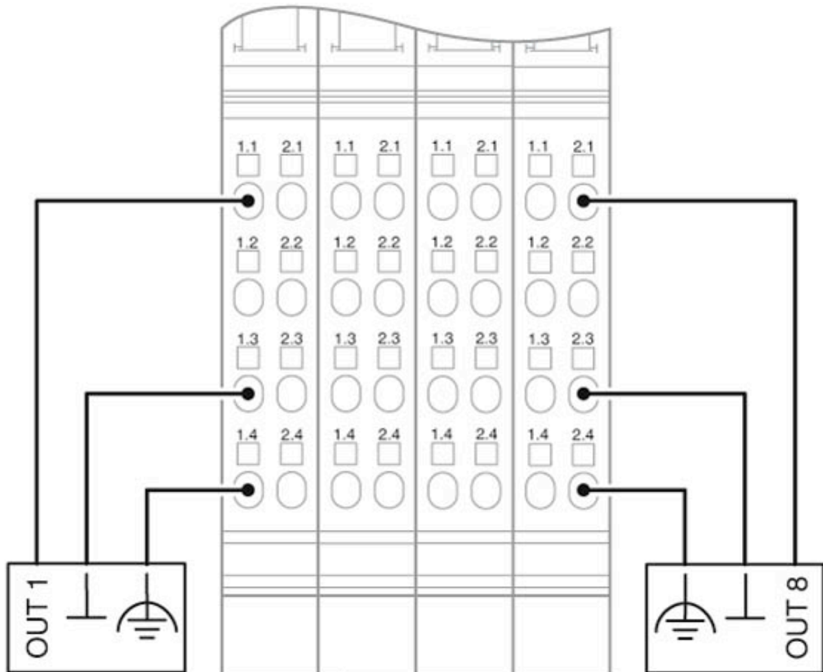
Connection diagram
