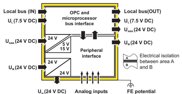
Figure 3 Electrical isolation of the individual function areas
