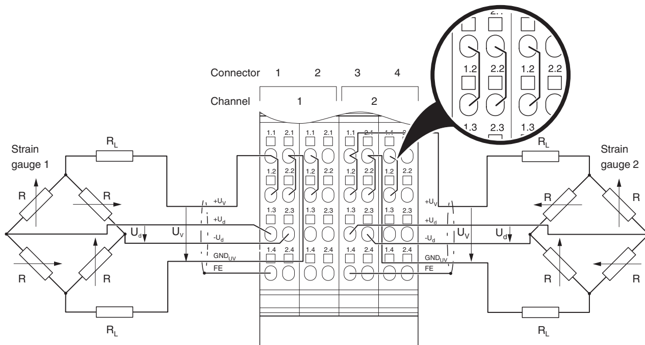
Figure 6 Connection of strain gauges in 4-wire technology (channel 1 and channel 2)
