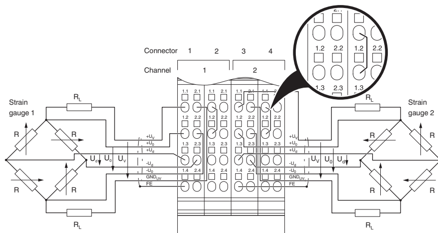
Figure 4 Connection of strain gauges in 6-wire technology
