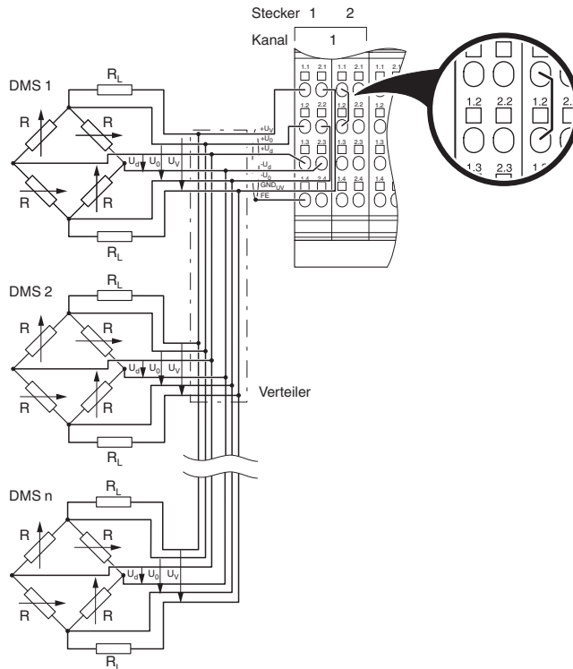
Figure 5 Connection of several strain gauges in 6-wire technology
