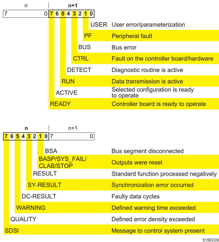
Figure 8 Diagnostic Status Register
