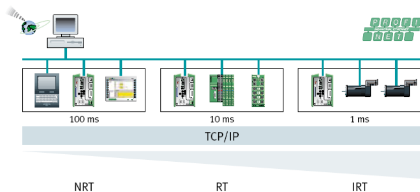
Figure 1-6 PROFINET- communication channels
