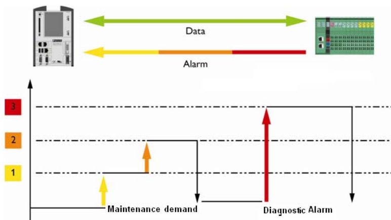
Figure 2-4 PROFINET diagnostic mechanisms
