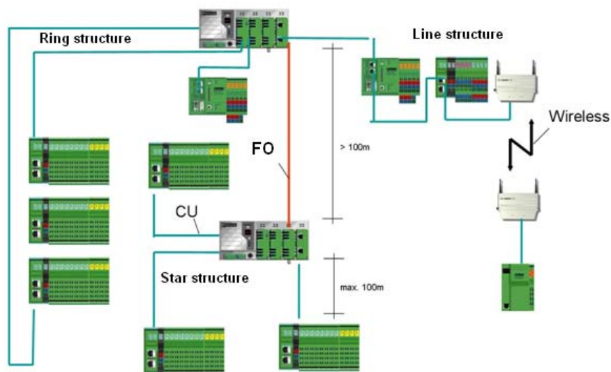
Figure 3-1 PROFINET topology example
