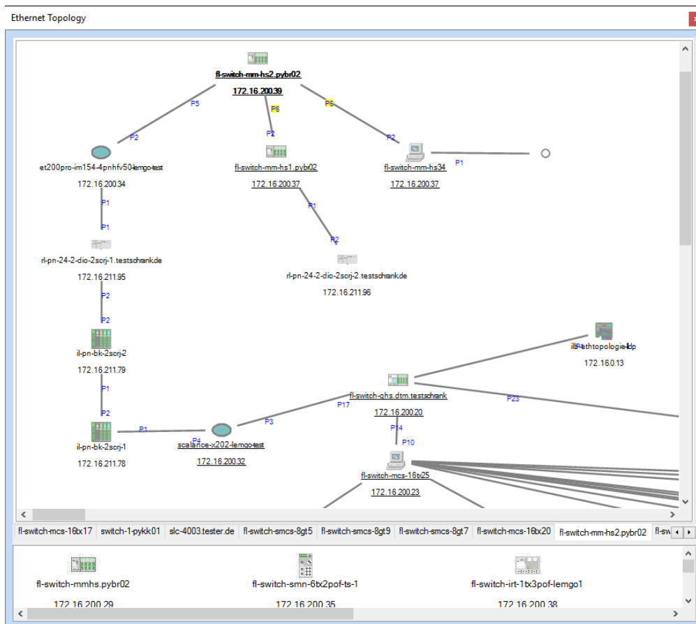
Figure 2-5 Topology detection
