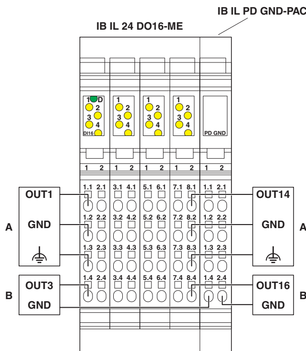
Figure 3 Typical connection of actuators when using the IB IL PD GND-PAC terminal
