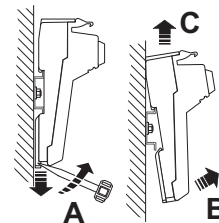
Figure 10-20 Removing the base
