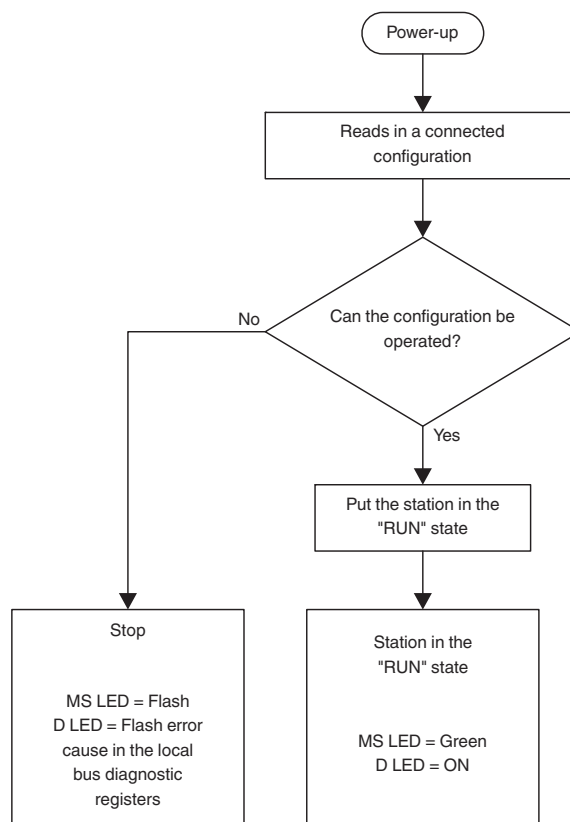
Figure 6 Plug and play mode activated
