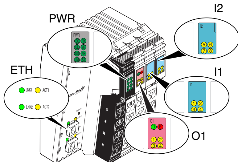
Figure 4 Local diagnostic and status indicators
