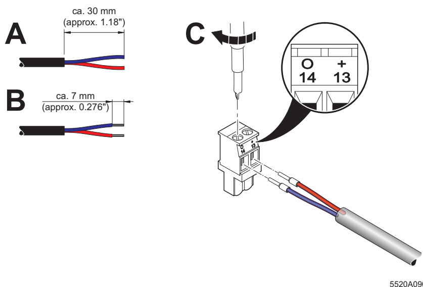
Figure 11-21 Assembling the connector for the brake
