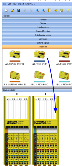
Figure 4-9 Hardware configuration
