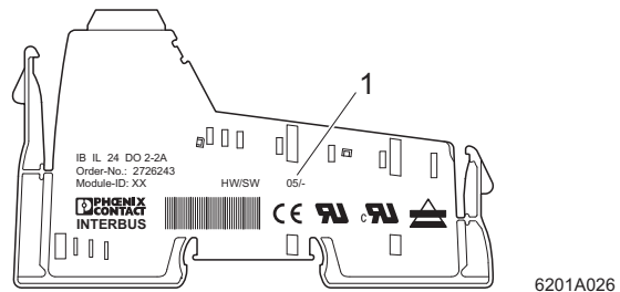
Figure 1 Printing on an Inline terminal
