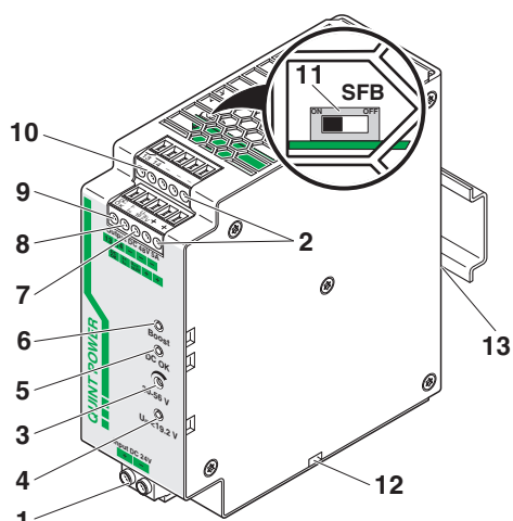
Figure 2 Function elements
