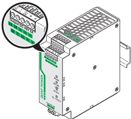
Figure 12 Signal outputs
