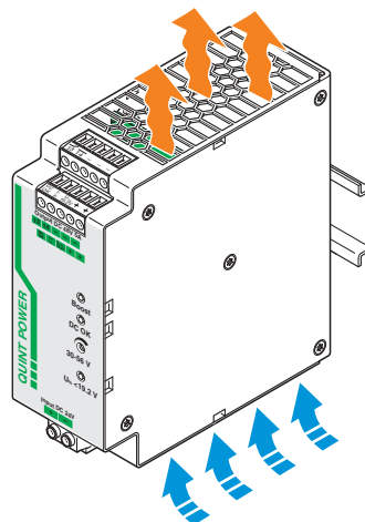
Figure 3 Convection
