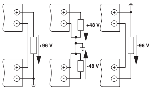
Figure 13 Series operation
