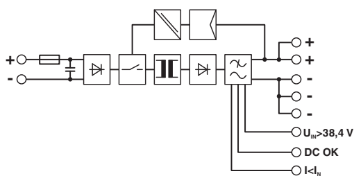
Figure 1 Block diagram
