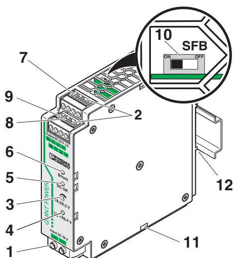
Figure 2 Function elements
