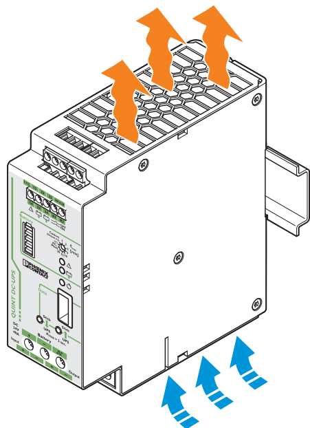
Figure 3 Convection
