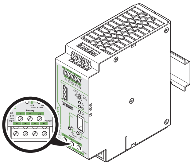
Figure 10 Output, battery
