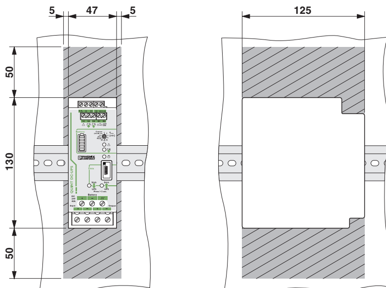
Figure 4 Installation dimensions
