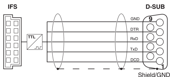
Figure 3 IFS-RS232-DATACABLE
