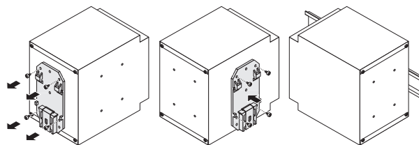
Figure 5 Schematic view of UTA change
