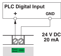
Figure 10 Power Good connection terminal blocks
