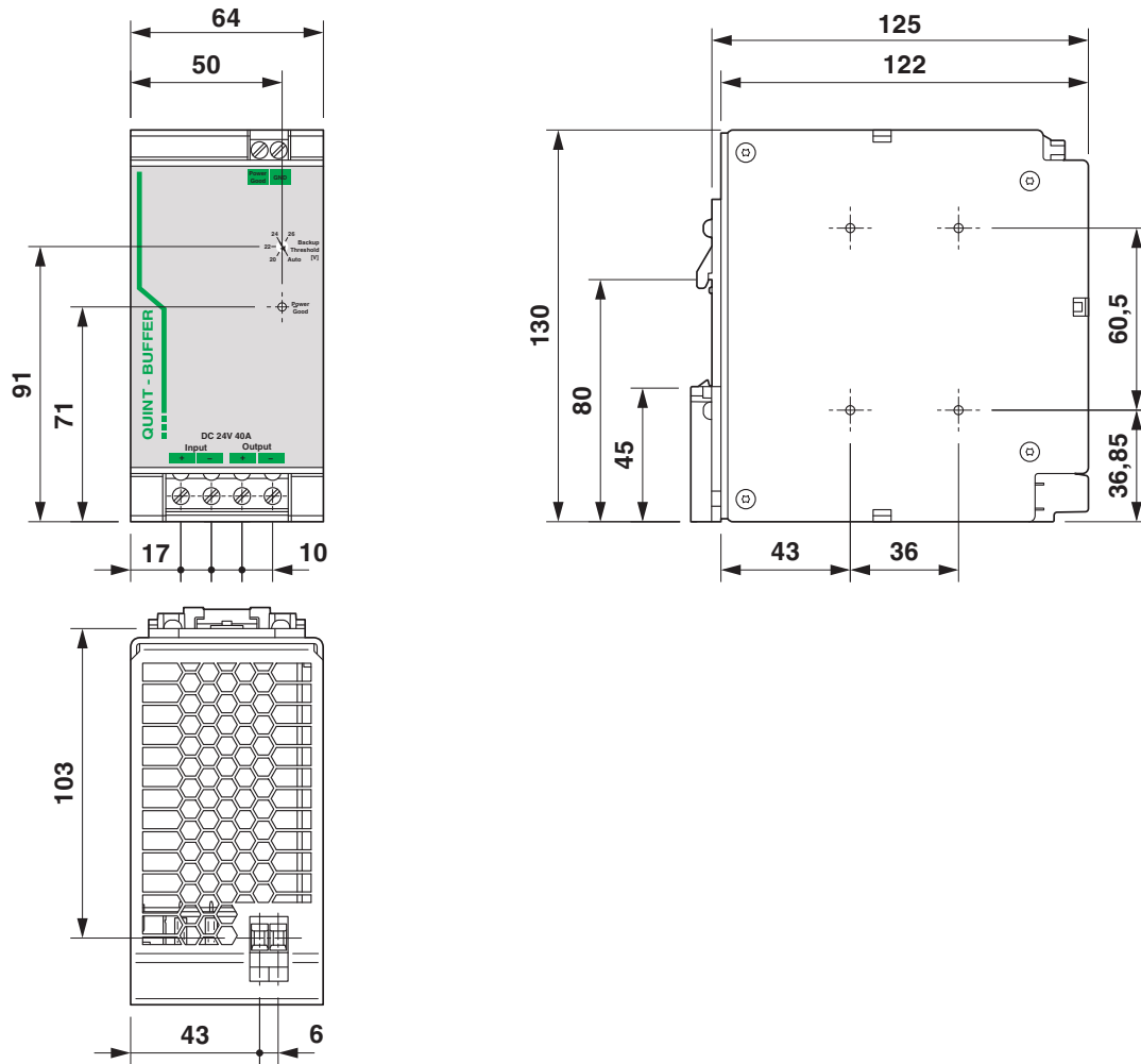
Figure 7 Device dimensions
