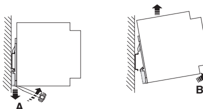
Figure 4 Removal
