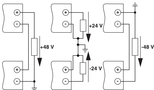
Figure 11 Series operation
