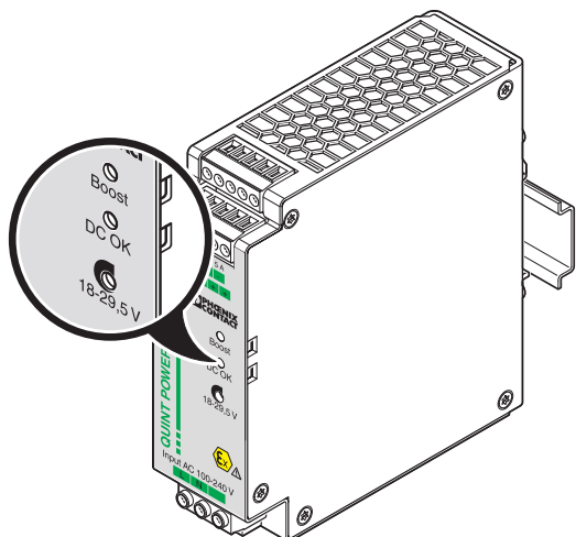
Figure 10 Signal outputs
