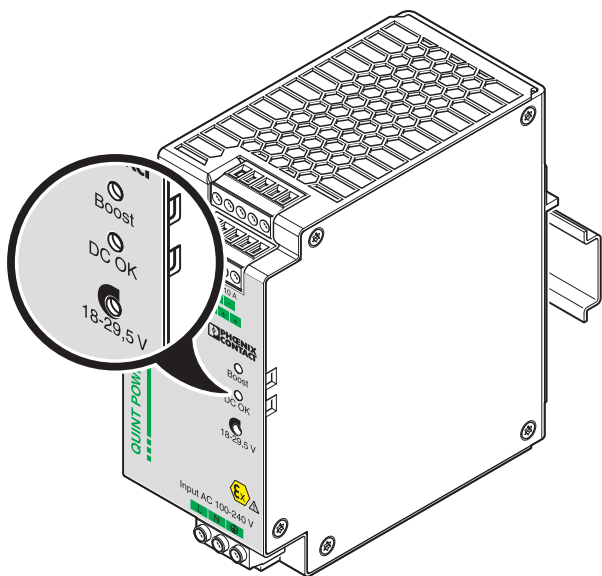
Figure 10 Signal outputs
