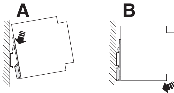
Figure 6 Assembly
