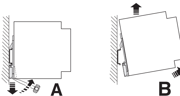
Figure 7 Removal
