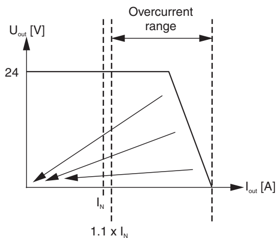
Figure 3-26 Fold-back characteristic
