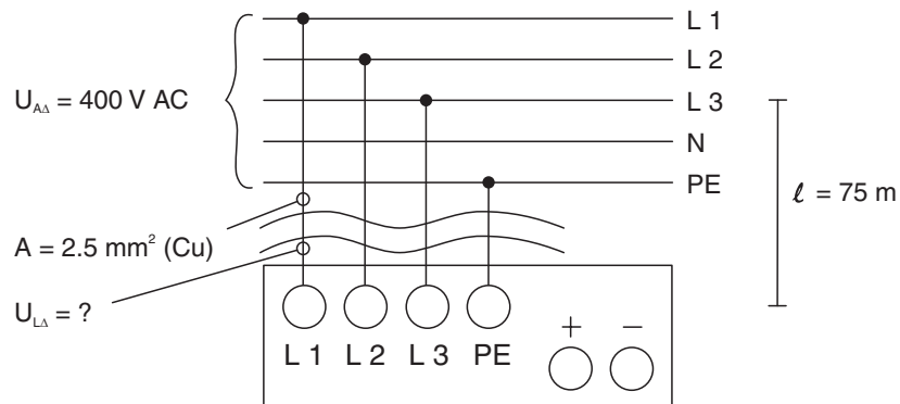
Figure 3-24 TN-S network
