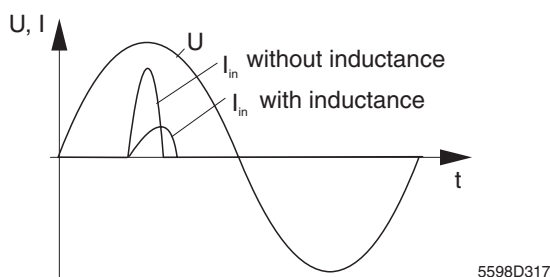
Figure 3-36 Harmonic filter
