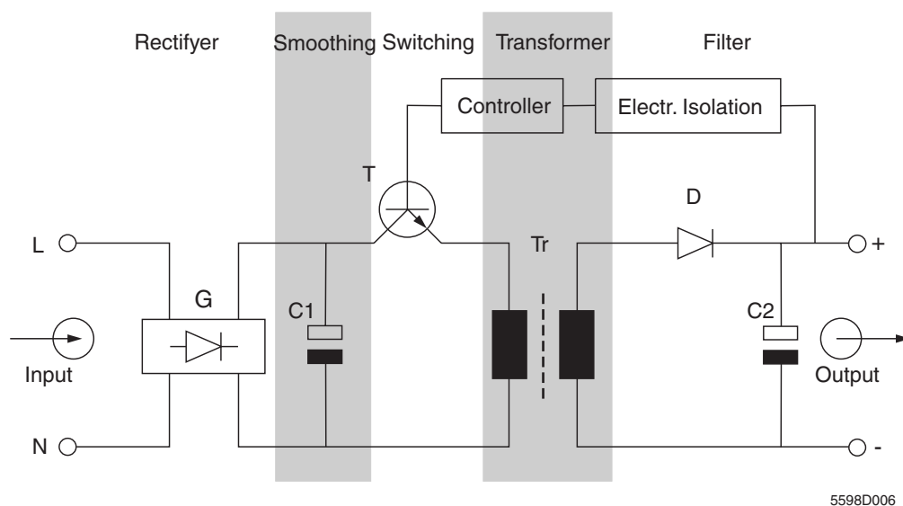
Figure 2-9 Circuit diagram for primary switched-mode devices
