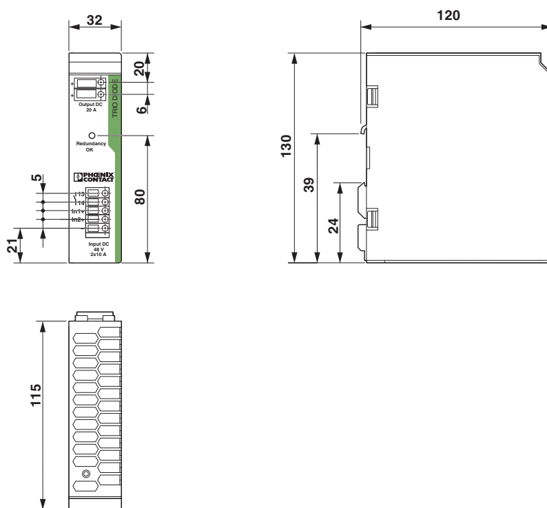
Figure 5 Device dimensions
