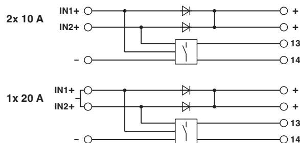
Figure 2 Block diagram
