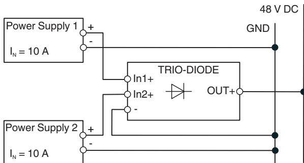
Figure 10 Decouple power supplies with nominal currents \leq 10 A
