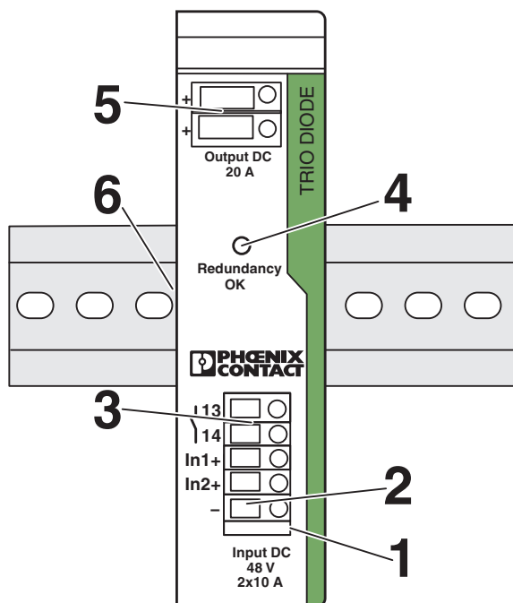
Figure 1 Device elements
