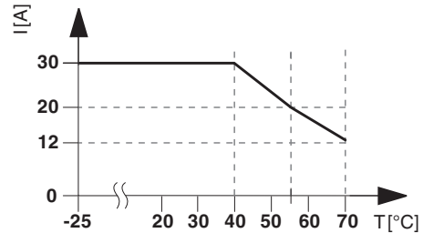
Figure 12 Temperature-dependent derating
