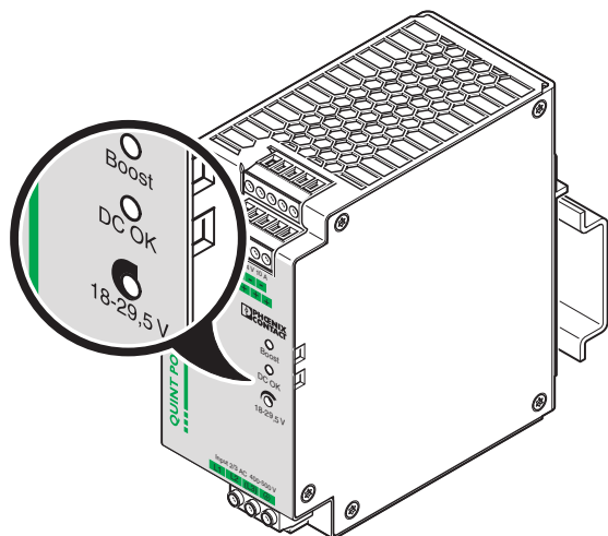
Figure 10 Signal outputs
