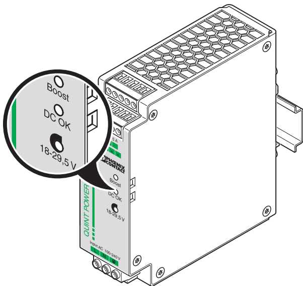
Figure 10 Signal outputs
