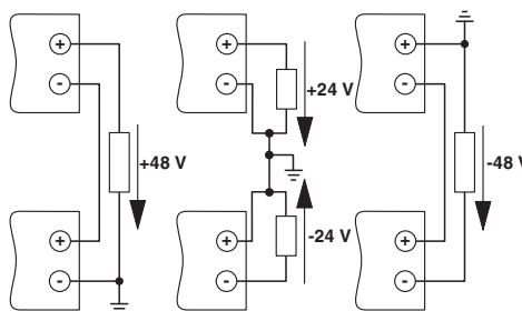
Figure 11 Series operation
