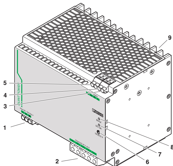
Figure 1 Position of the function elements
