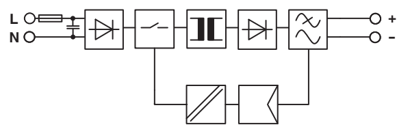
Figure 2 Block diagram
