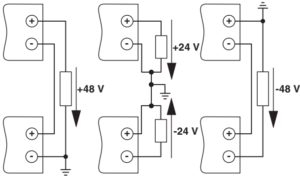
Figure 17 Series operation
