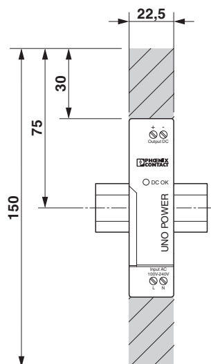
Figure 4 Device dimensions and dead surfaces
