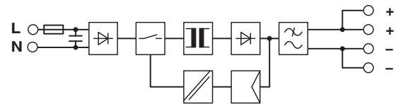
Figure 2 Block diagram
