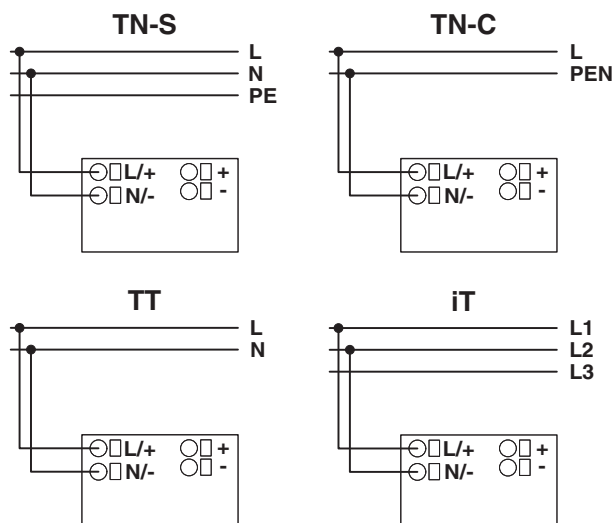
Figure 10 Network types
