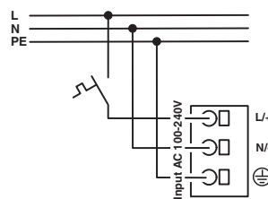
Figure 12 Schematic diagram, switching the input terminals
