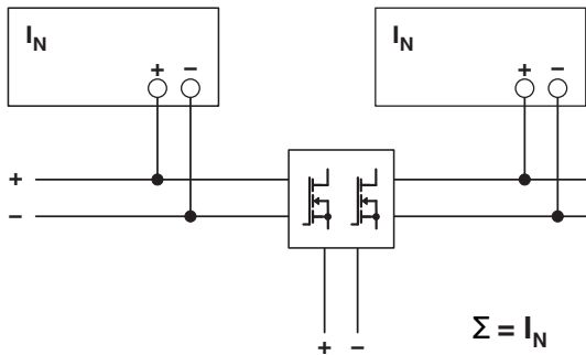
Figure 46 Schematic diagram, redundant operation with QUINT ORING
