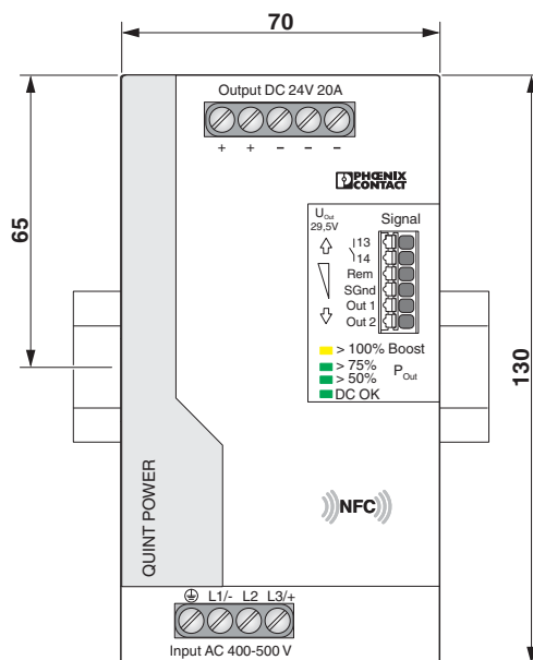
Figure 4 Device dimensions (dimensions in mm)
