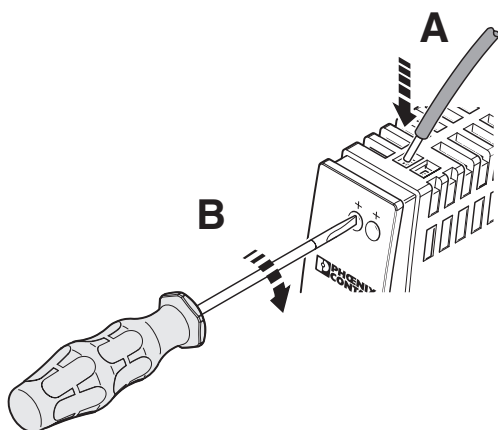
Figure 16 Connecting cables
