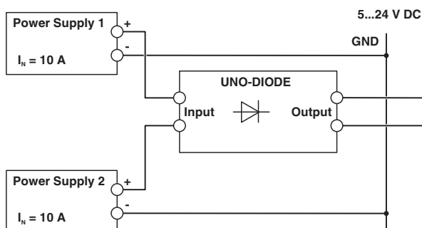
Figure 17 Decouple power supplies with nominal currents ≤ 10 A
