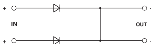
Figure 2 Block diagram
