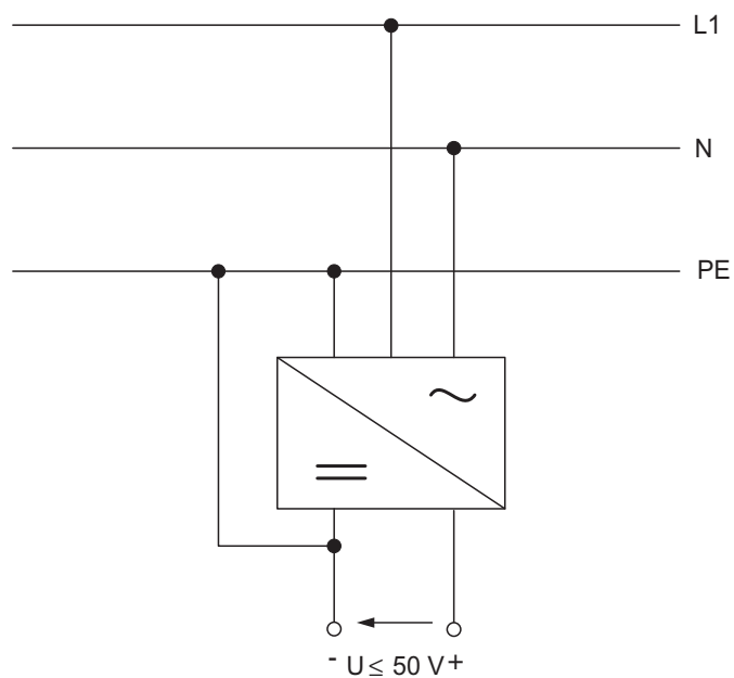
Figure 2-6 Secondary protection
