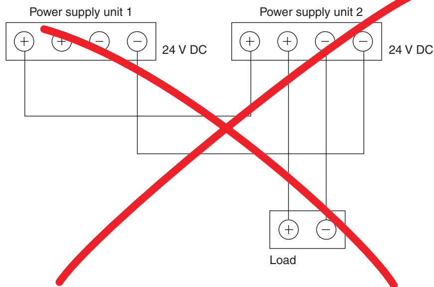
Figure 3-6 Incorrect parallel connection in the secondary circuit
