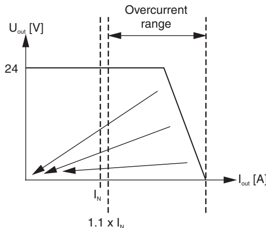
Figure 3-26 Fold-back characteristic
