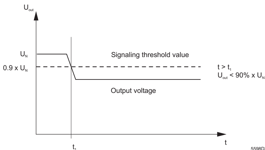
Figure 3-11 Output voltage not OK
