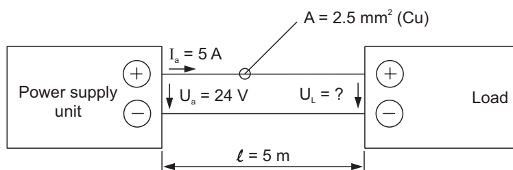
Figure 3-23 Voltage across the load
