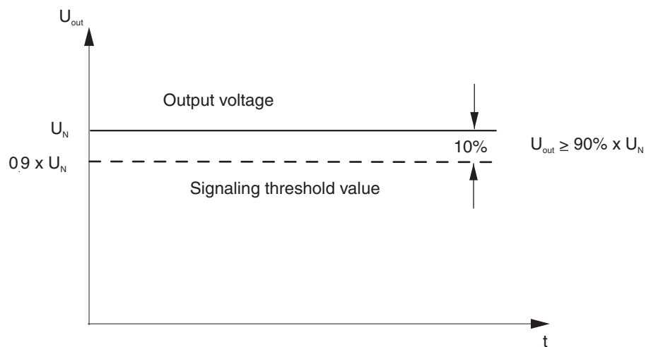
Figure 3-10 Output voltage OK
