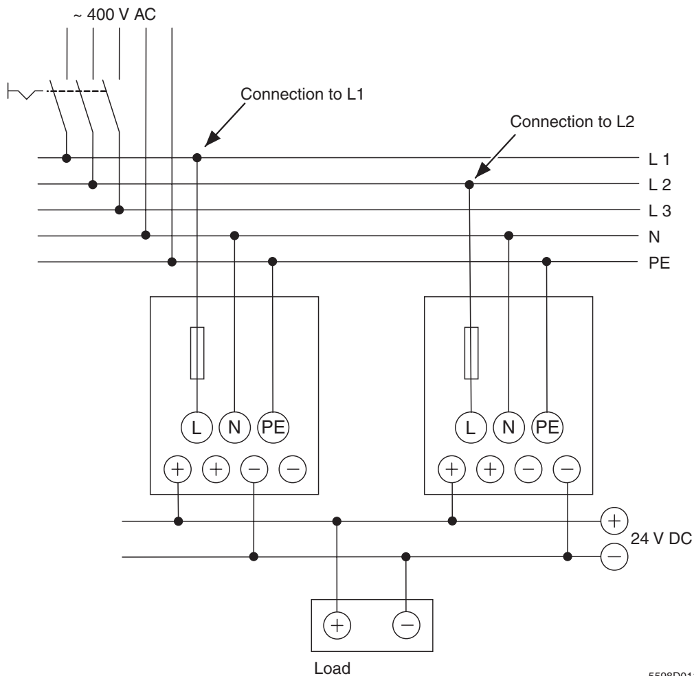
Figure 3-7 One-phase redundancy operation
