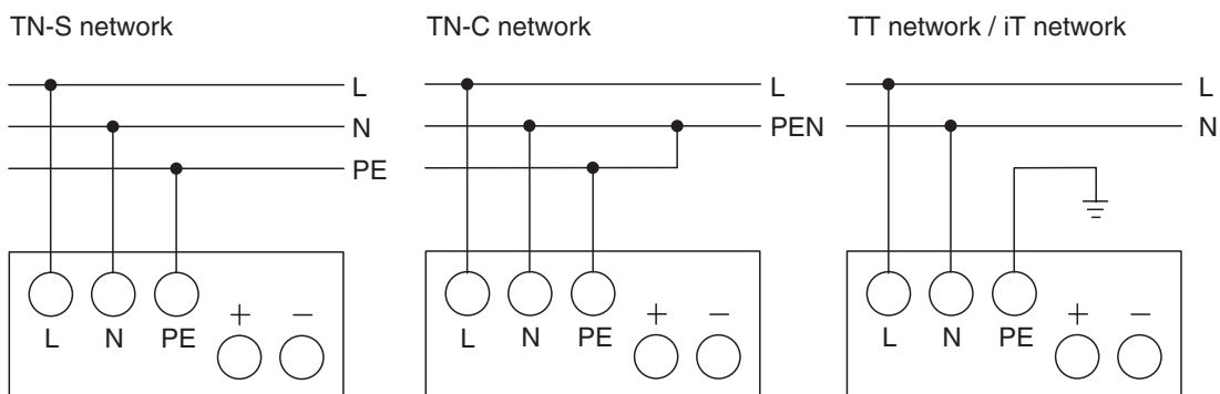
Figure 3-17 Connection of a one-phase power supply unit
