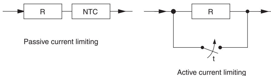
Figure 3-25 Current limiting
