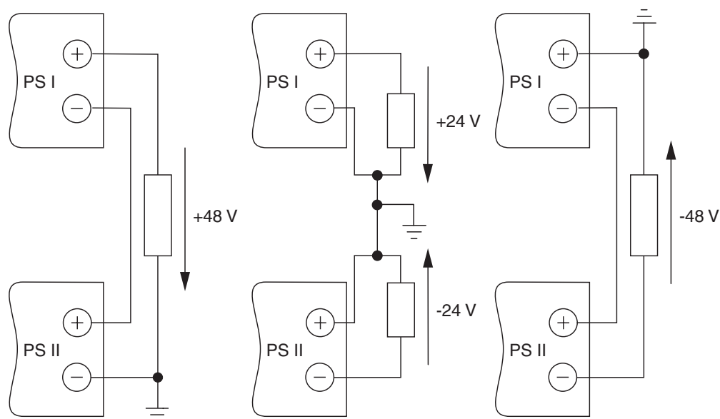
Figure 3-9 Series connection
