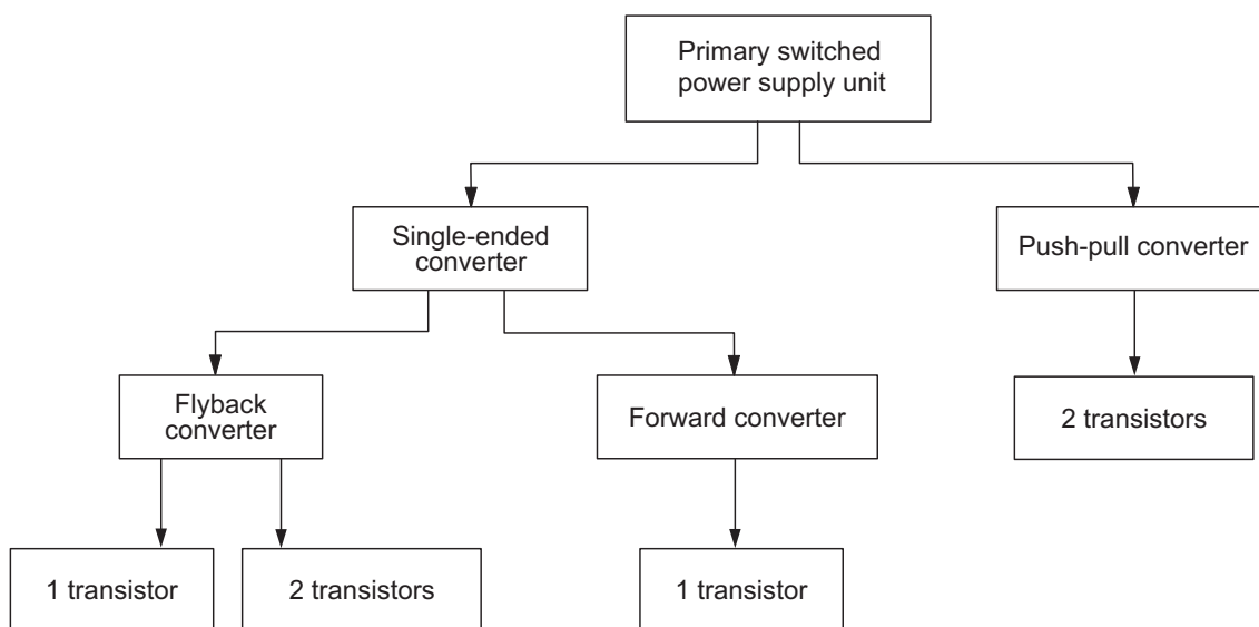
Figure 2-11 Converter types
