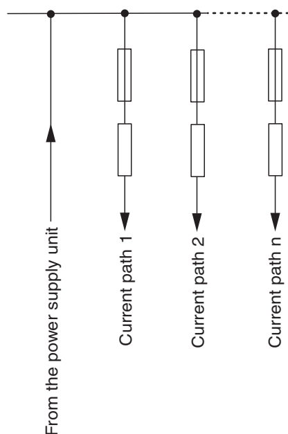
Figure 3-21 Selective protection
