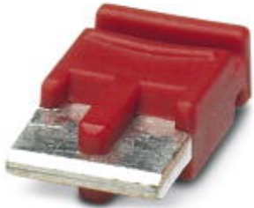
Single plug-in bridge, length: 6 mm, number of positions: 2, color: red
