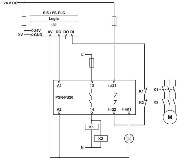
Figure 14 High-demand application with failsafe controller
