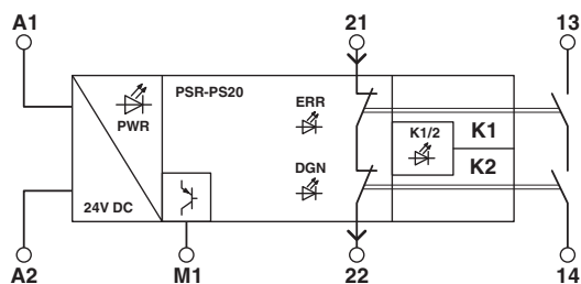
Figure 3 Block diagram
