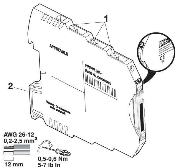
Figure 8 Connection versions
