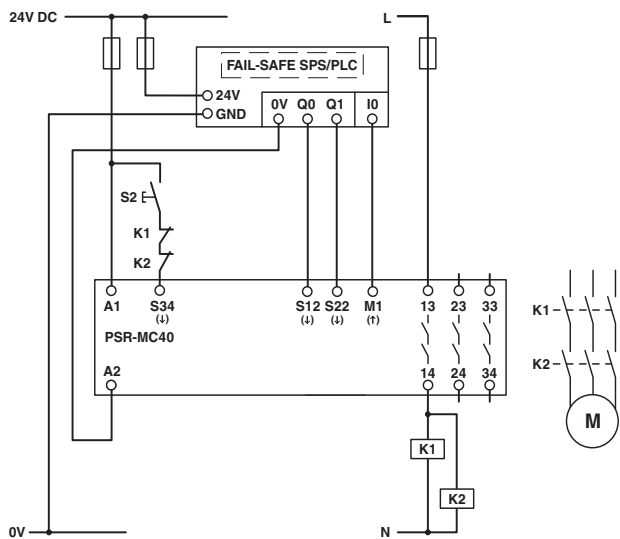
Figure 56 Connection to failsafe PLC/manual, monitored start
