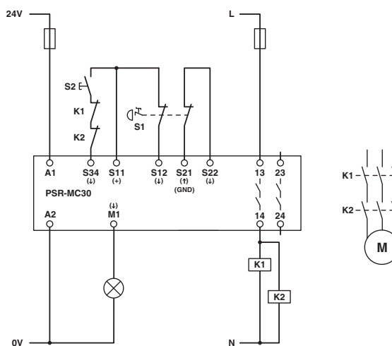
Figure 30 Emergency stop monitoring/manual, monitored start
