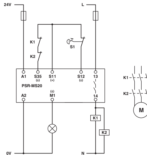
Figure 1 Emergency stop monitoring/automatic start
