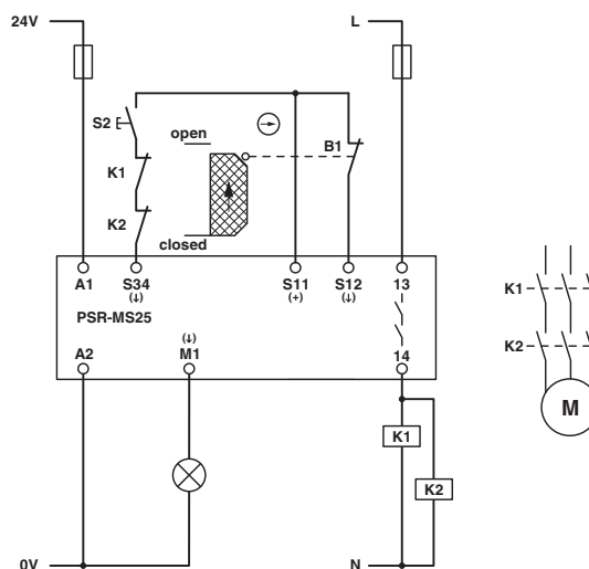
Figure 5 Safety door monitoring/manual, monitored start
