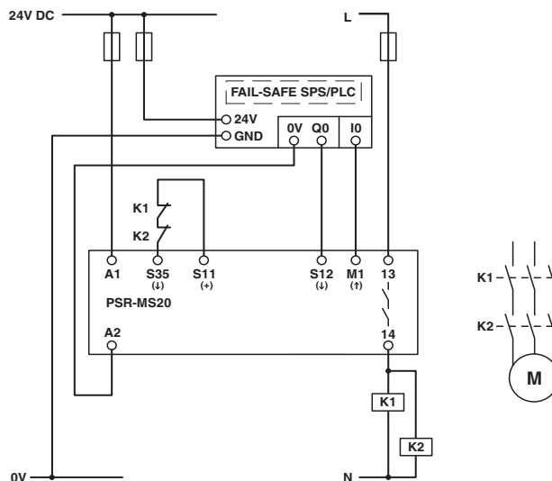
Figure 3 Connection to failsafe PLC/automatic start
