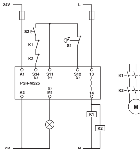
Figure 4 Emergency stop monitoring/manual, monitored start
