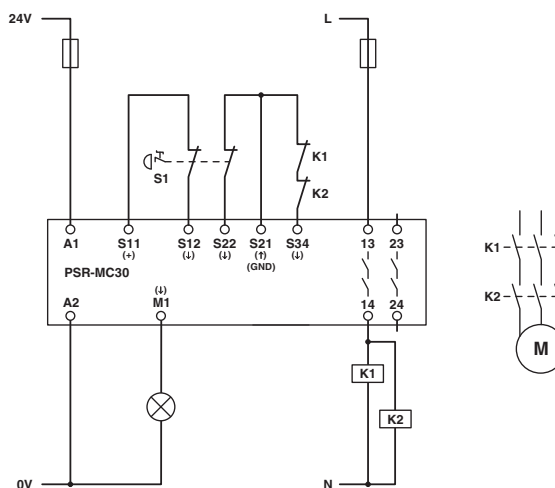
Figure 29 Emergency stop monitoring/automatic start
