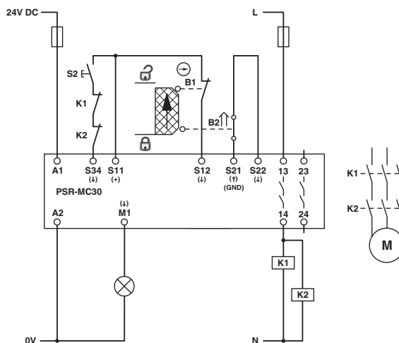
Figure 17 Safety door monitoring/manual, monitored start
