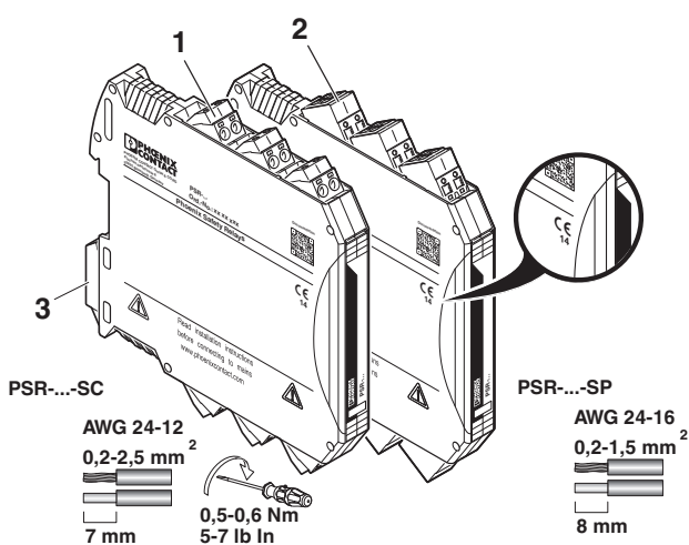
Figure 6 Connection versions
