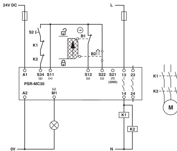
Figure 18 Safety door monitoring/manual, monitored start/without cross-circuit detection
