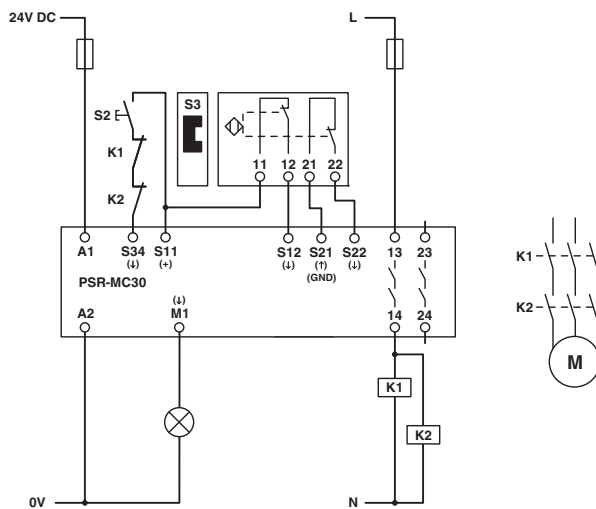
Figure 21 Magnetic switch monitoring/manual, monitored start
