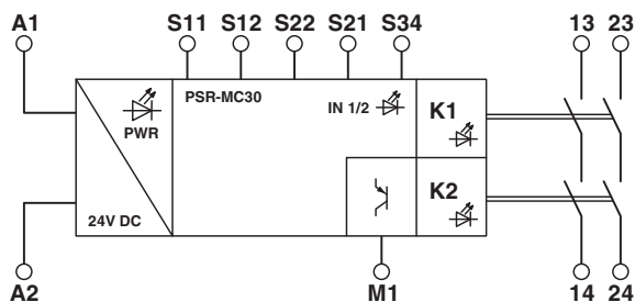
Figure 3 Block diagram
