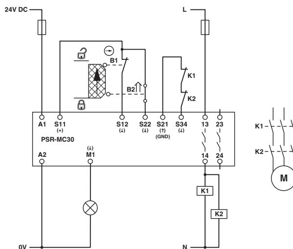
Figure 15 Safety door monitoring/automatic start/without cross-circuit detection
