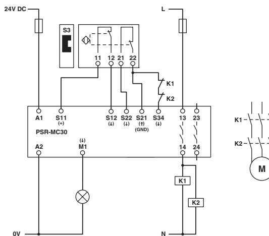
Figure 20 Magnetic switch monitoring/automatic start
