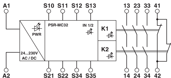
Figure 4 Block diagram
