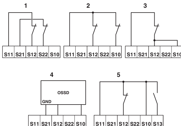
Figure 13 Signal generator connection versions
