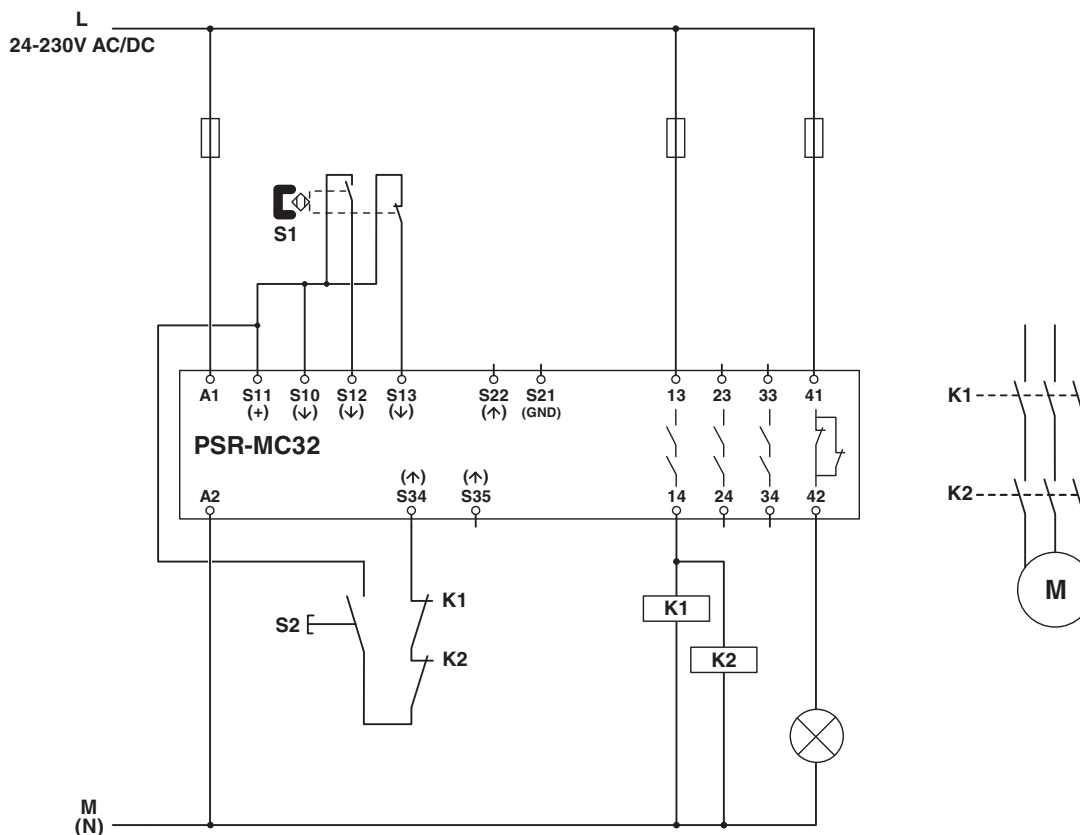
Figure 21 Magnetic switch monitoring/manual, monitored start
