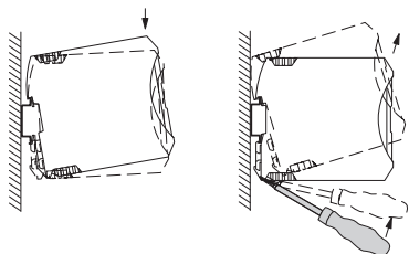
Figure 10 Mounting and removing
