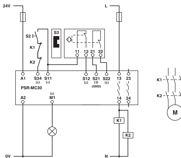
Figure 38 Magnetic switch monitoring/manual, monitored start
