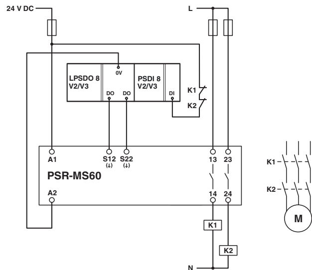
Figure 22 Two-channel control via LPSDO module
