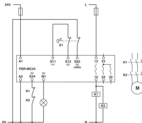
Figure 39 Emergency stop monitoring/automatic start
