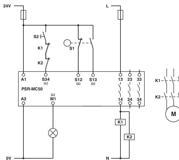
Figure 66 Safety door monitoring/manual, monitored start
