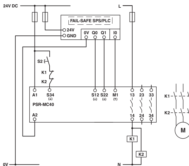
Figure 56 Connection to failsafe PLC/manual, monitored start
