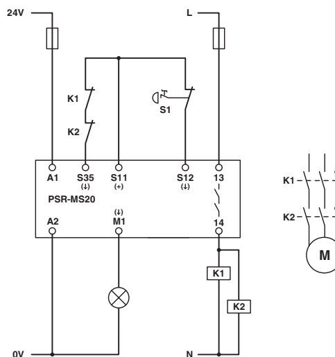
Figure 1 Emergency stop monitoring/automatic start
