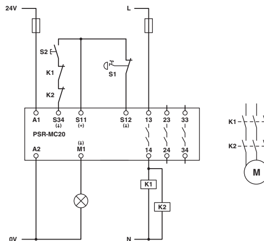
Figure 25 Emergency stop monitoring/manual, monitored start
