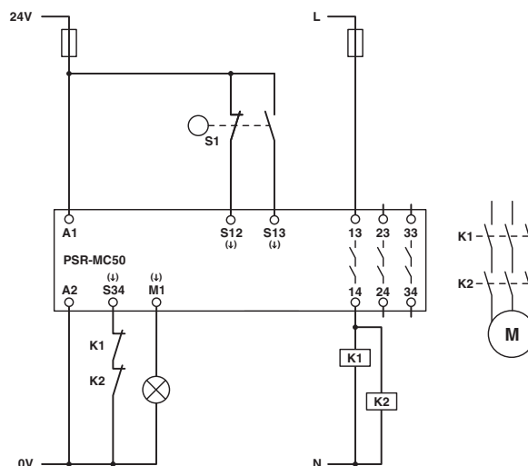
Figure 65 Safety door monitoring/automatic start
