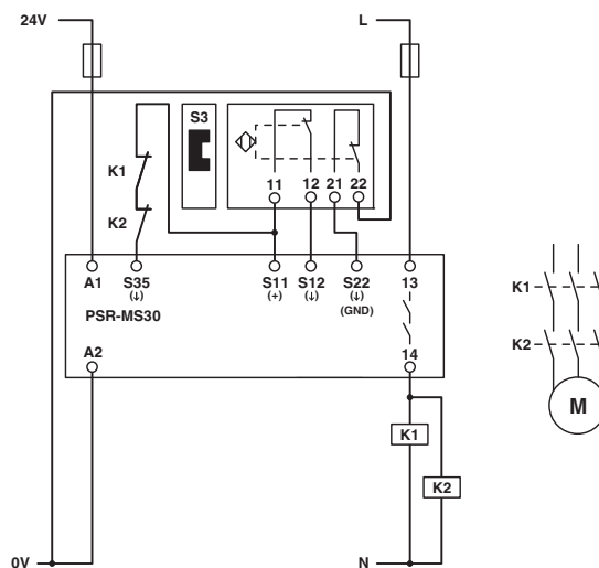
Figure 9 Magnetic switch monitoring/automatic start
