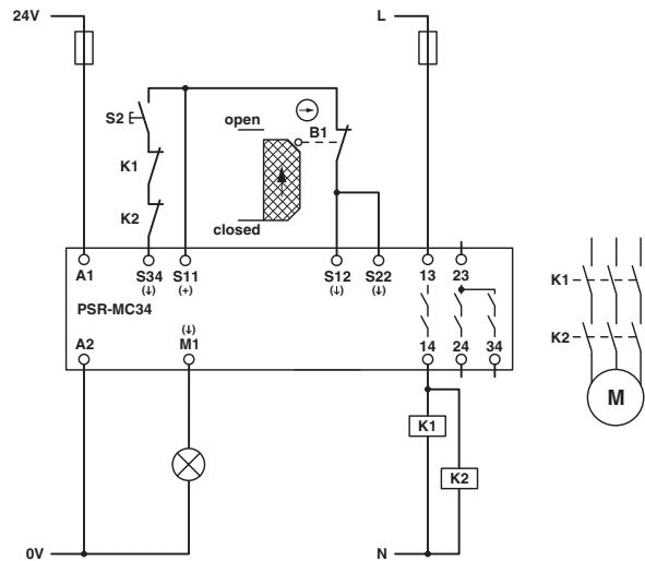
Figure 46 Single-channel safety door monitoring/manual, monitored start
