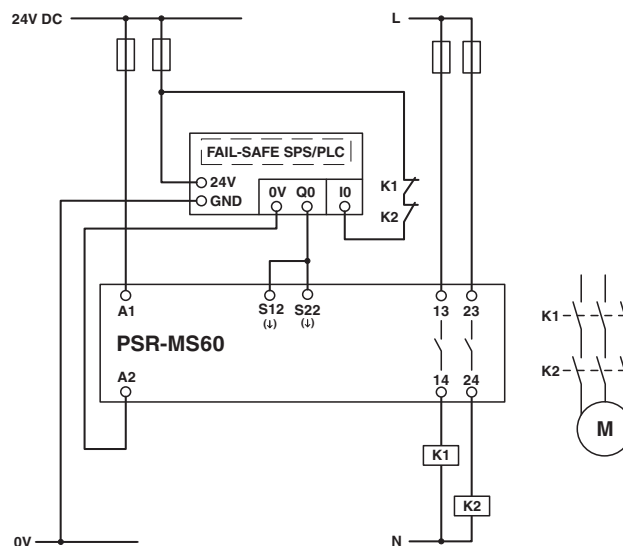
Figure 23 Single-channel control via failsafe PLC
