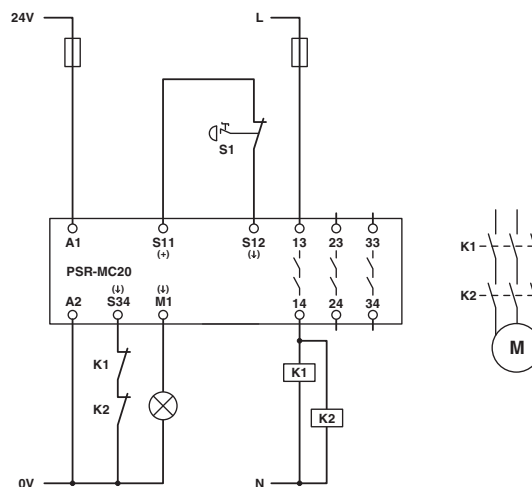
Figure 24 Emergency stop monitoring/automatic start
