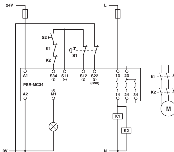
Figure 40 Emergency stop monitoring/manual, monitored start
