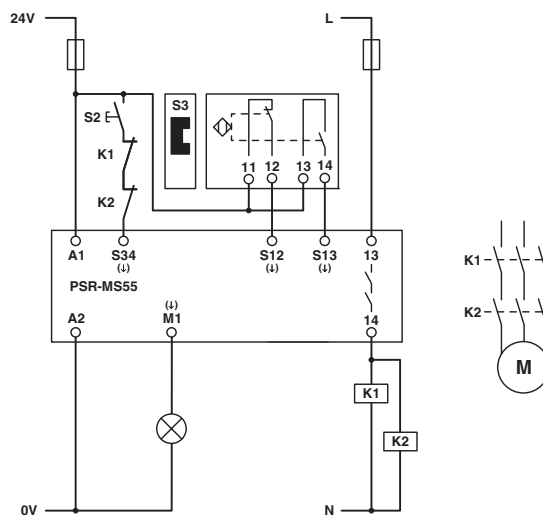
Figure 20 Magnetic switch monitoring/manual, monitored start
