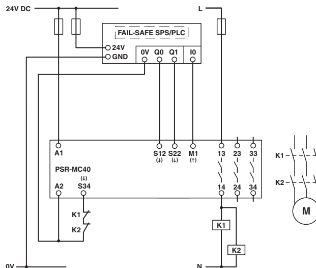
Figure 55 Connection to failsafe PLC/automatic start
