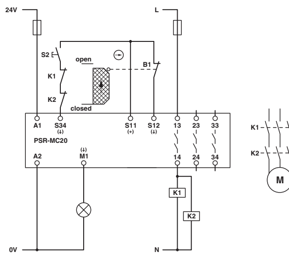
Figure 27 Safety door monitoring/manual, monitored start
