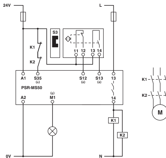
Figure 19 Magnetic switch monitoring/automatic start
