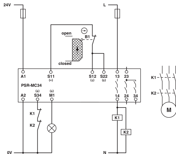
Figure 43 Single-channel safety door monitoring/automatic start
