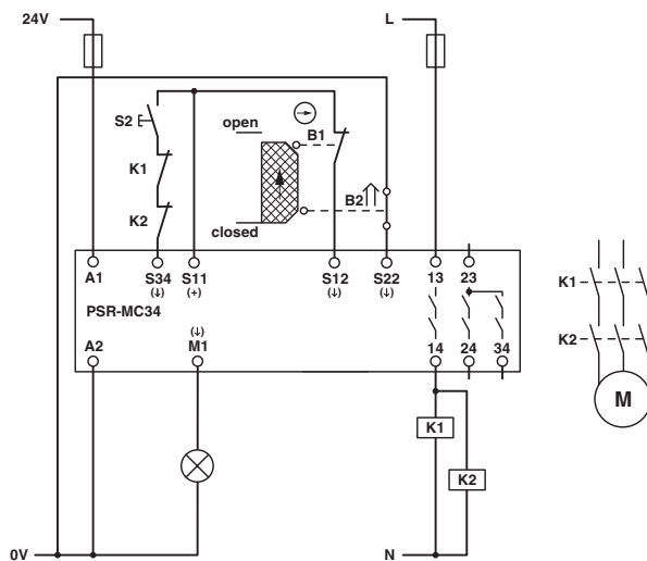
Figure 44 Safety door monitoring/manual, monitored start
