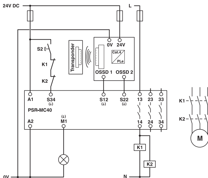
Figure 25 Transponder monitoring/manual, monitored start
