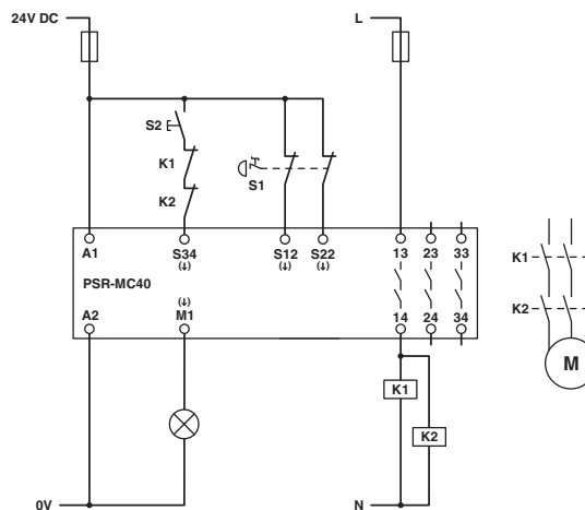
Figure 13 Emergency stop monitoring/manual, monitored start
