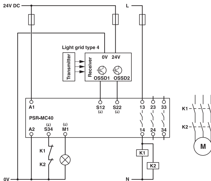
Figure 22 Light grid monitoring/automatic start
