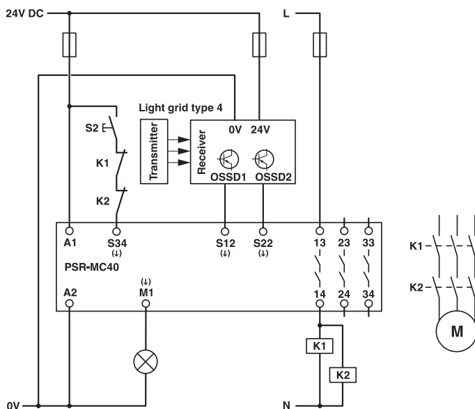
Figure 23 Light grid monitoring/manual, monitored start
