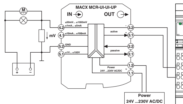
Figure 6 Example, shunt measurement
