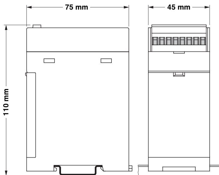
Figure 1 Dimensions
