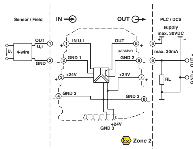
Figure 3 Block diagram
