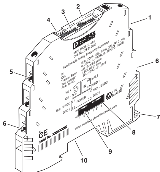
Figure 2 Structure
