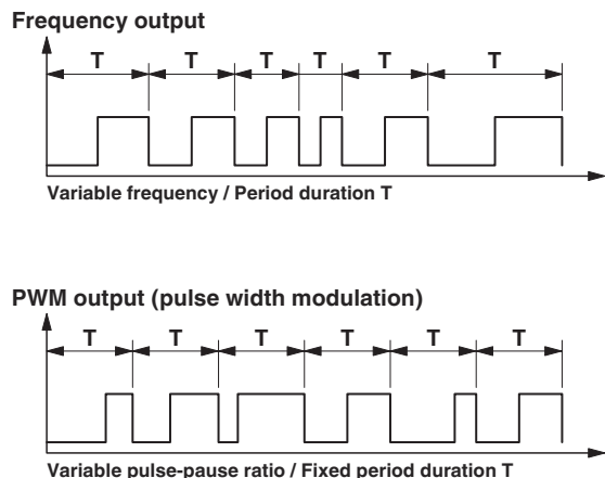
Figure 8 Output signals
