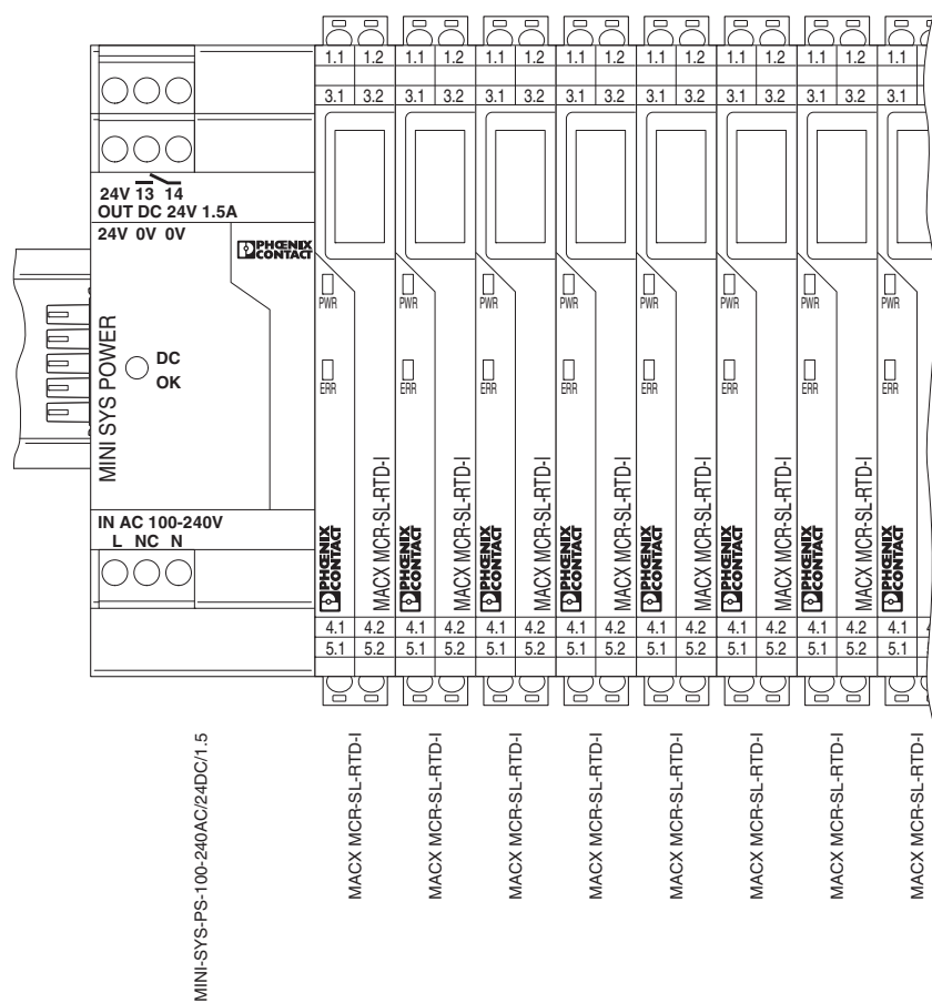
Figure 5-11 Example for supply via a system power supply
