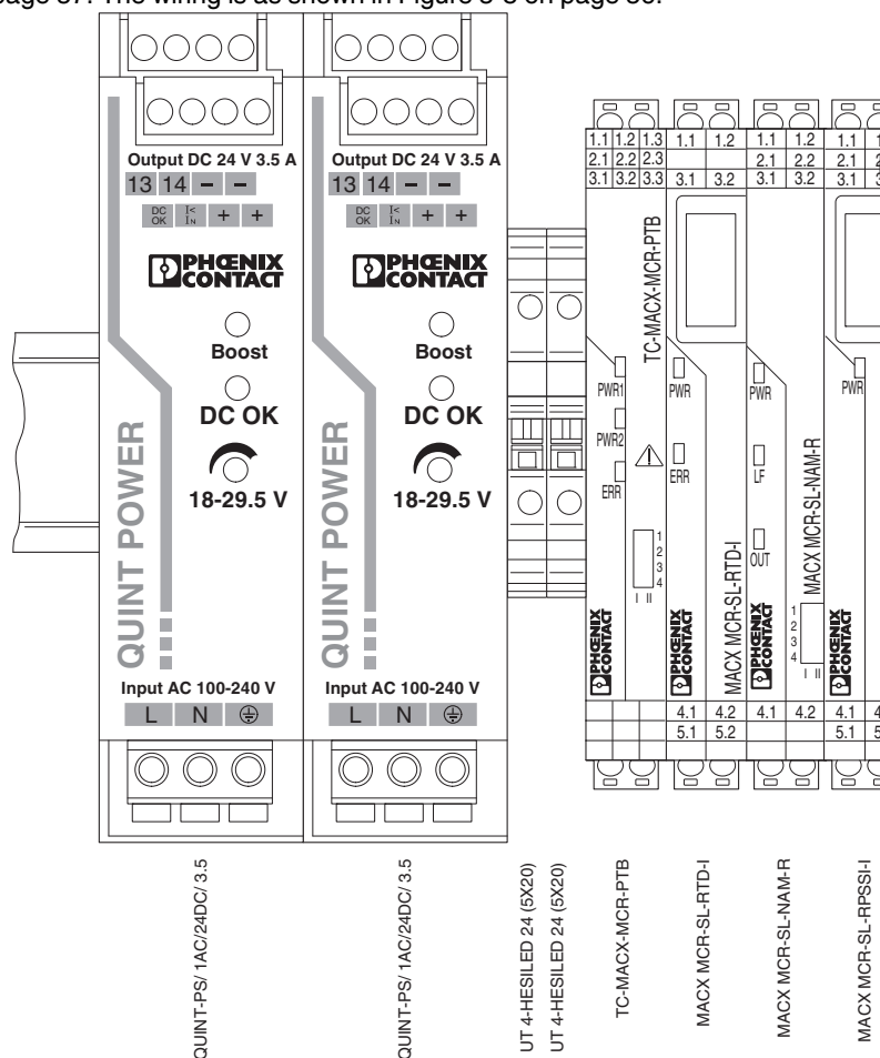
Figure 5-9 Example for supply via a TC-MACX-MCR-PTB power terminal block
