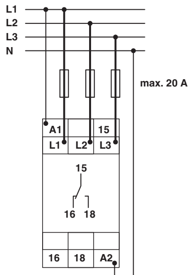
3 ~ 400 V measuring range with 230 V AC power module
