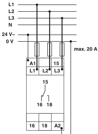
3 ~ 400 V measuring range with 24 V AC power module
